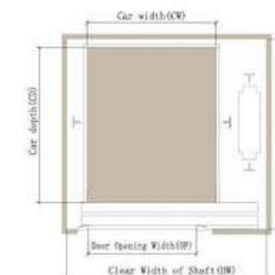
Shaft plan for Side opening door
