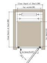
Backpack rack (Manually-operated door)
