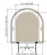
Horseshoe shaped sightseeing elevator (automatic exterior door)
