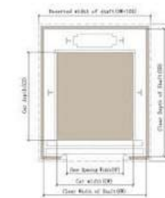
Shaft plan for Center-opening bi-folding door
