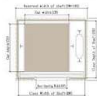
Shaft plan for Center opening door
