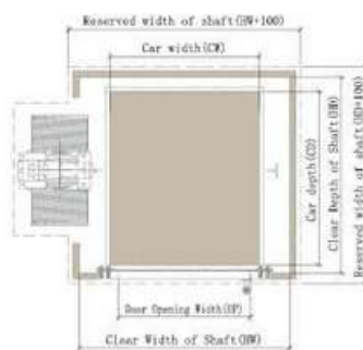
Shaft plan for the Downward drum drive
