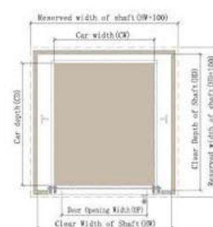
Shaft plan for the Top-mounted drum drive
