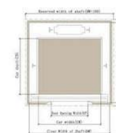
Shaft plan for Center opening door
